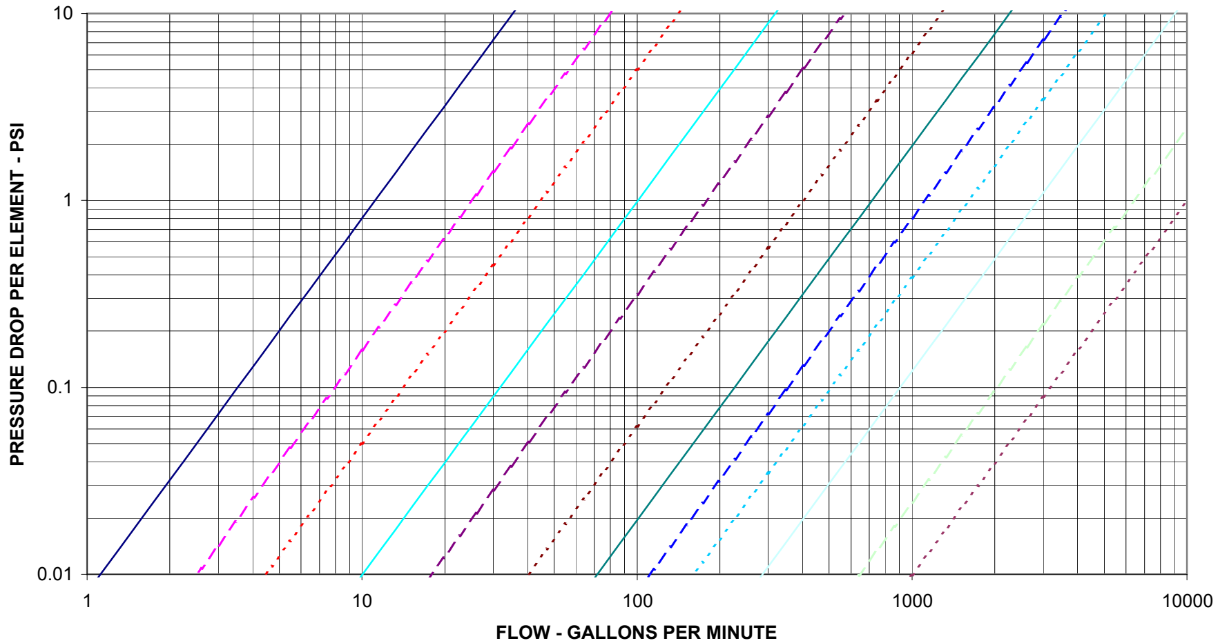
FIGURE 2 - LPD TURBULENT FLOW SP. GR. = 1; VISC. = 1 CPS
