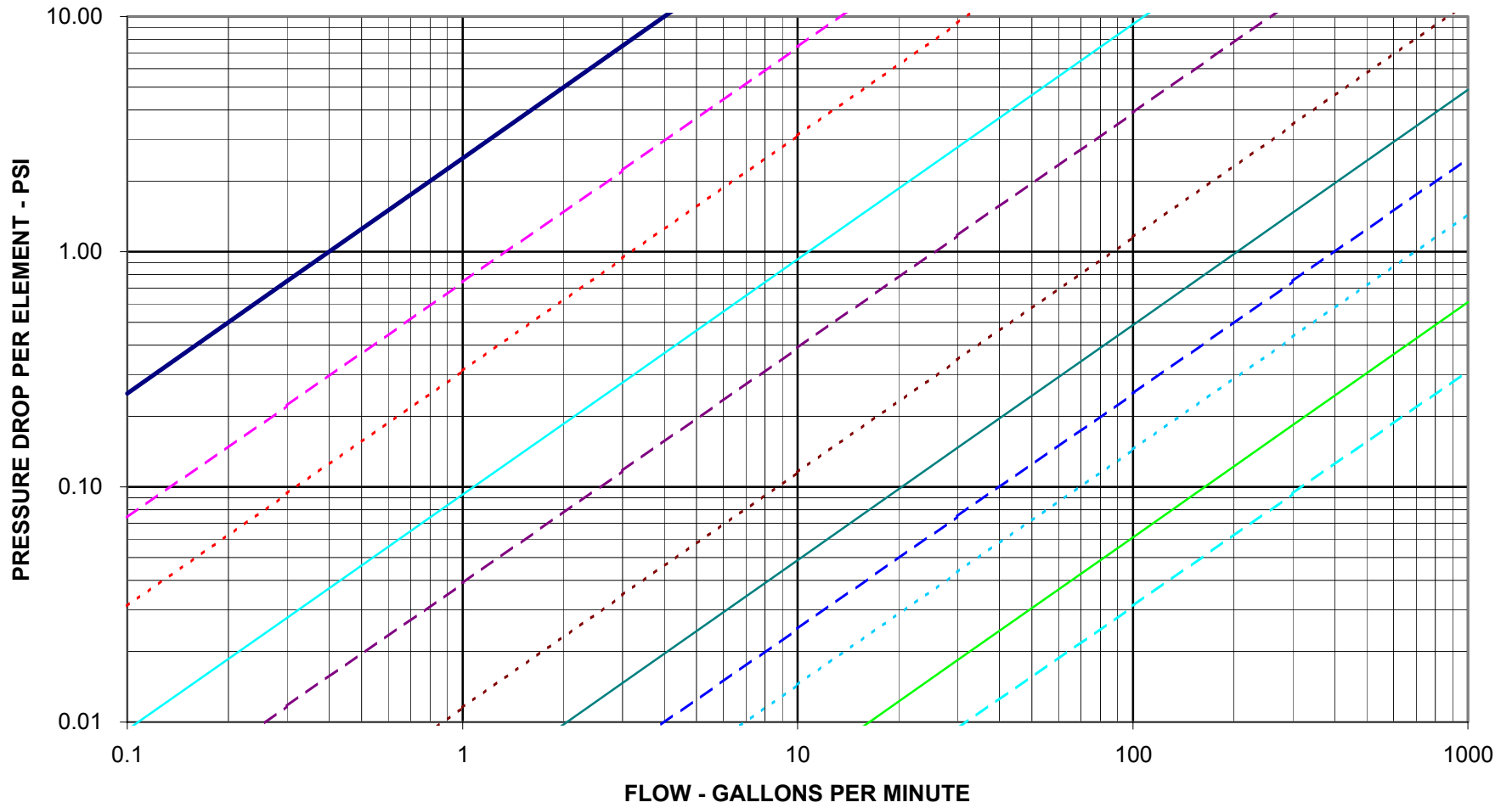
FIGURE 1 - LPD LAMINAR FLOW - VISCOSITY 10,000 CPS
