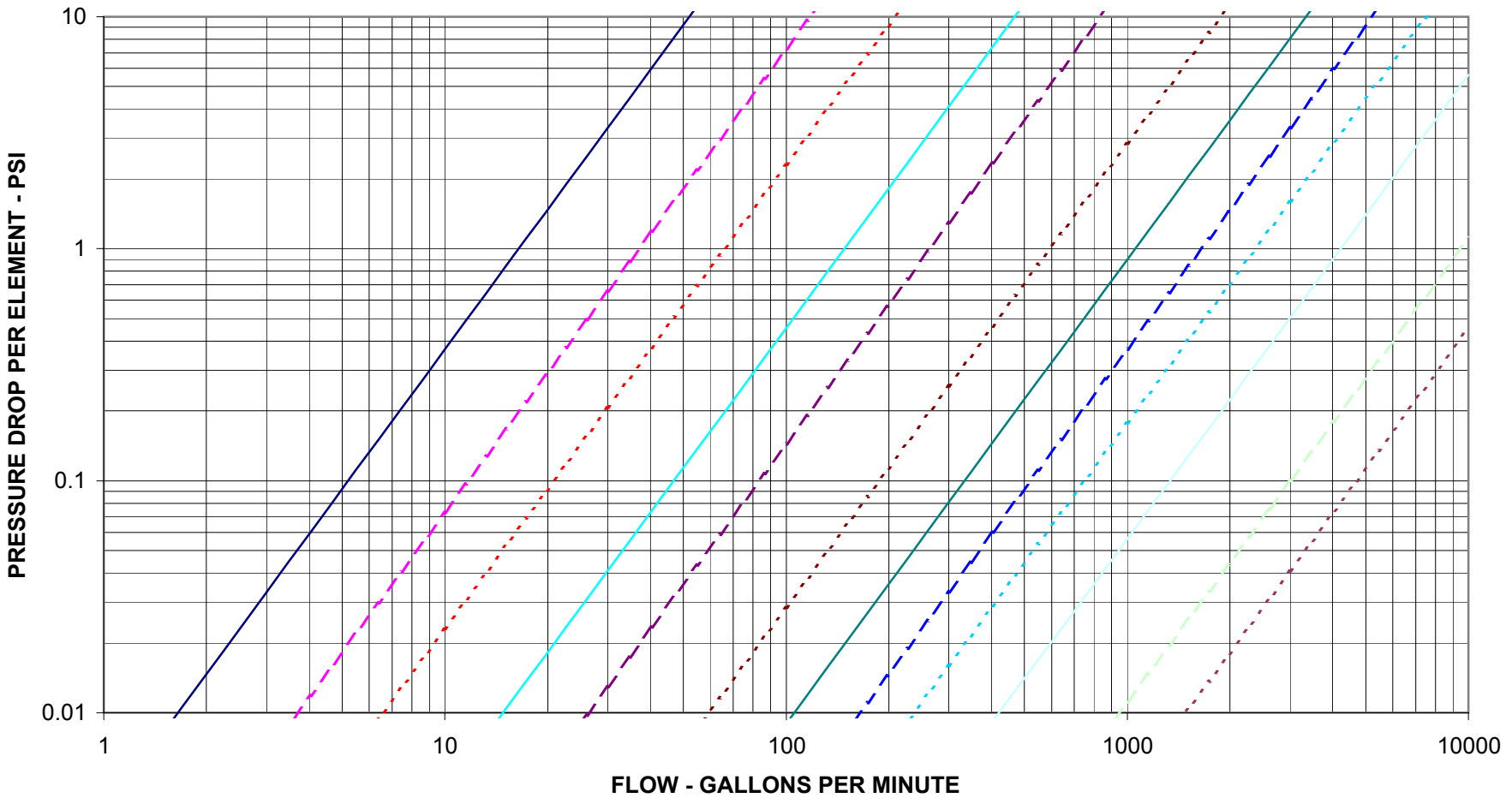
FIGURE 4 - LLPD TURBULENT FLOW SP. GR. = 1; VISC. = 1 CPS
