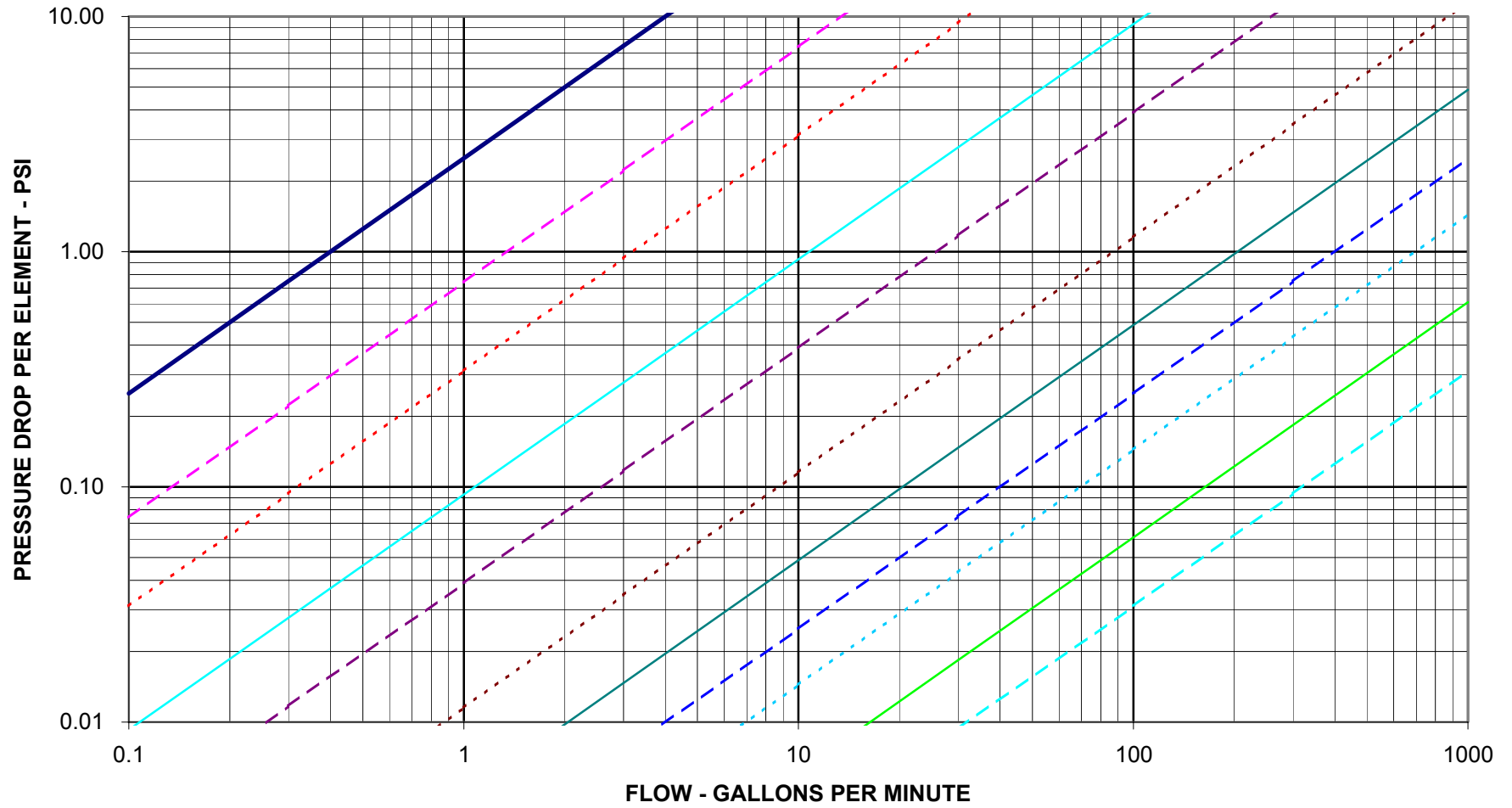
FIGURE 3 - LLPD LAMINAR FLOW - VISCOSITY 10,000 CPS
