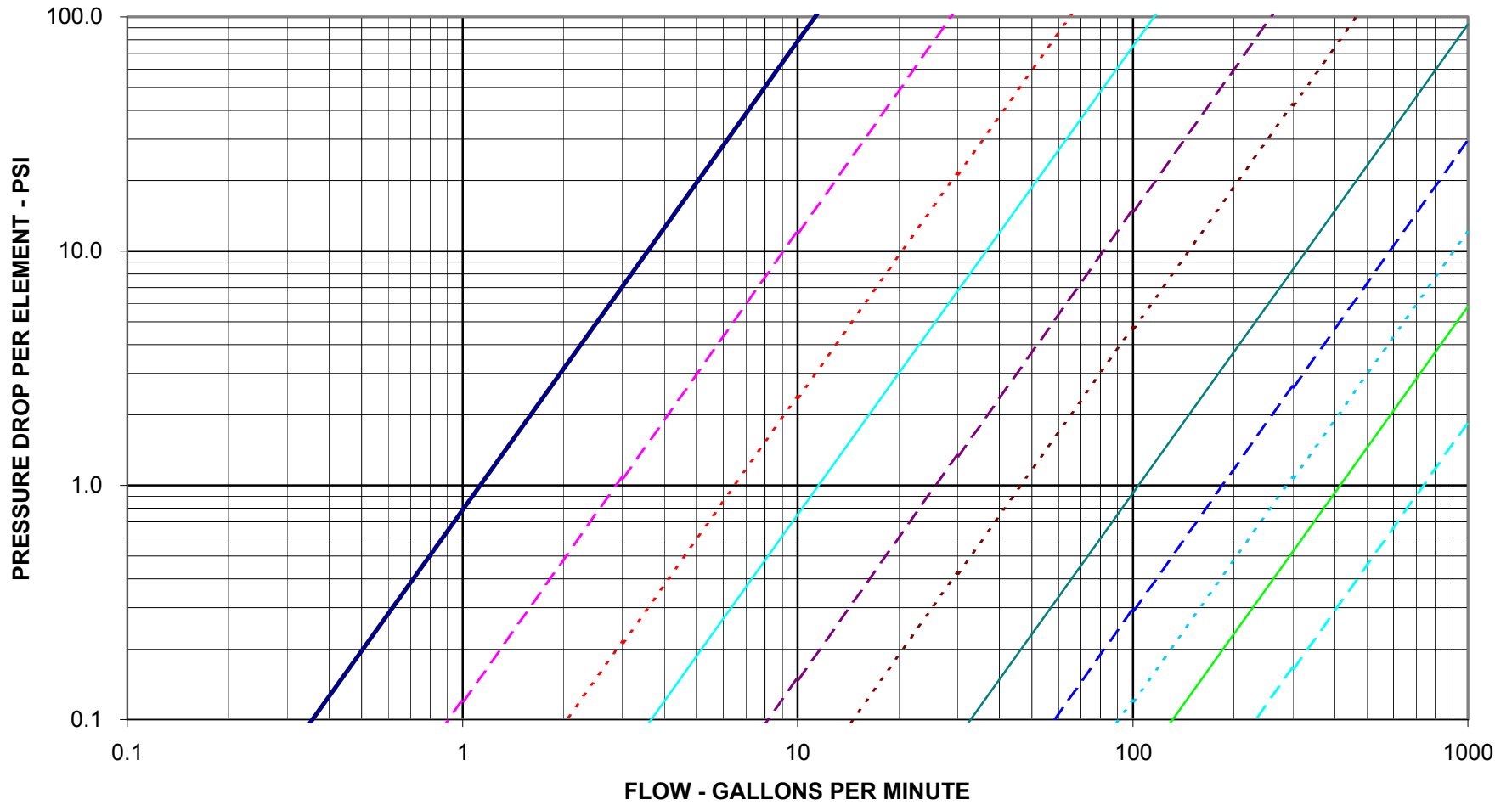
FIGURE 6 - ISG TURBULENT FLOW SP. GR. = 1; VISC. = 1 CPS
