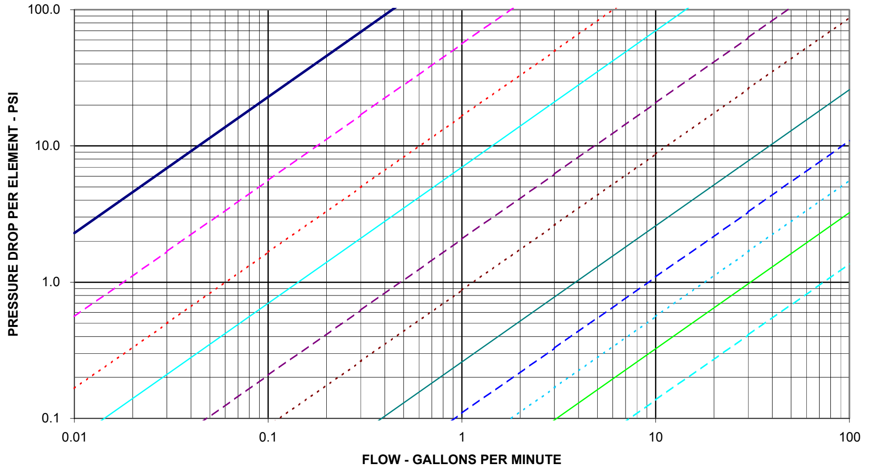
FIGURE 5 - ISG LAMINAR FLOW - VISCOSITY 10,000 CPS
